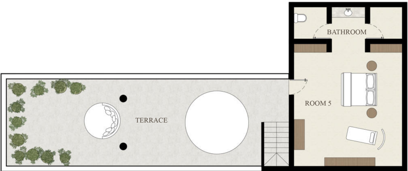
SECOND FLOOR
